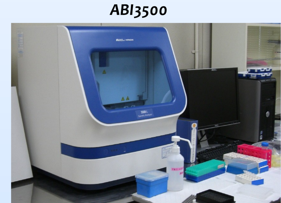
Capillary Electrophoresis
